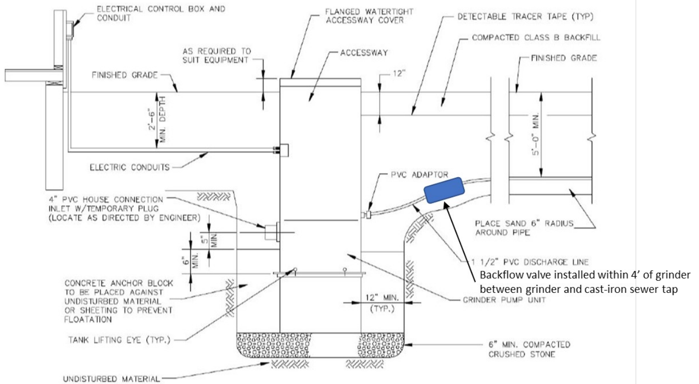
TYPICAL GRINDER PUMP INSTALLATION
